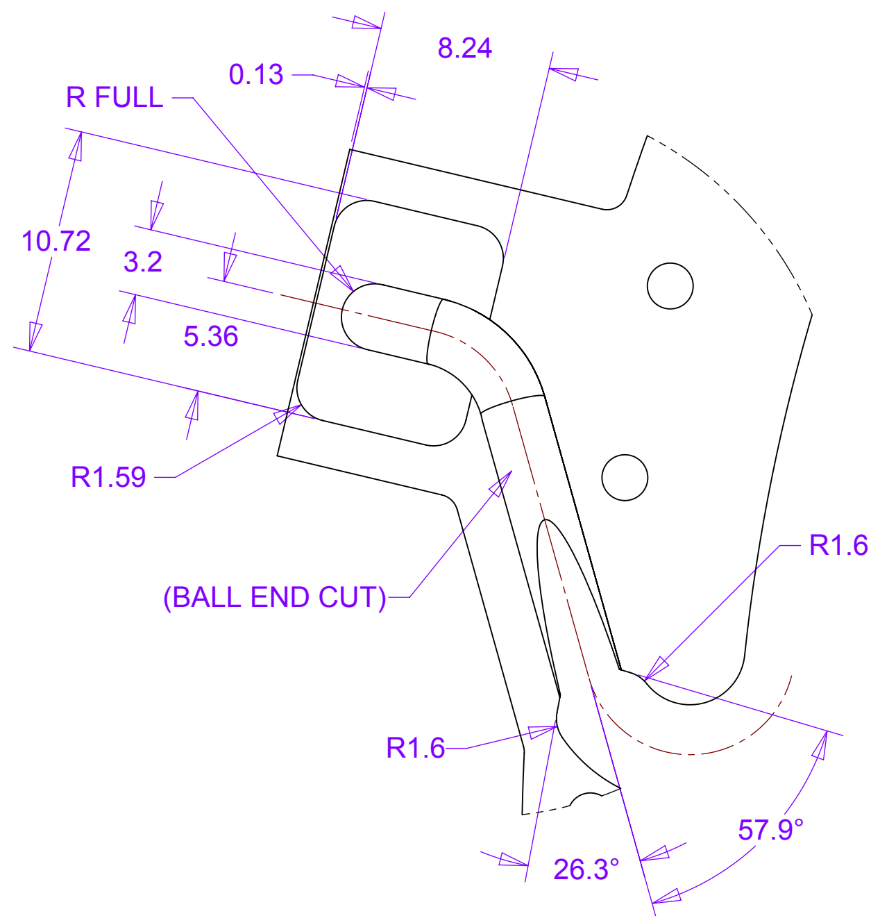
DETAIL K
