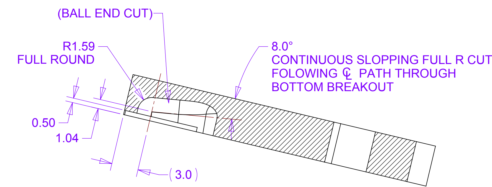
SECTION F-F
